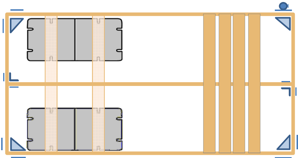
Example : 6' x 12' Semi-Floating
